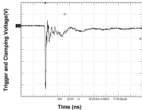
Fig.6 IEC61000-4-2 -8kV Contact Discharge
