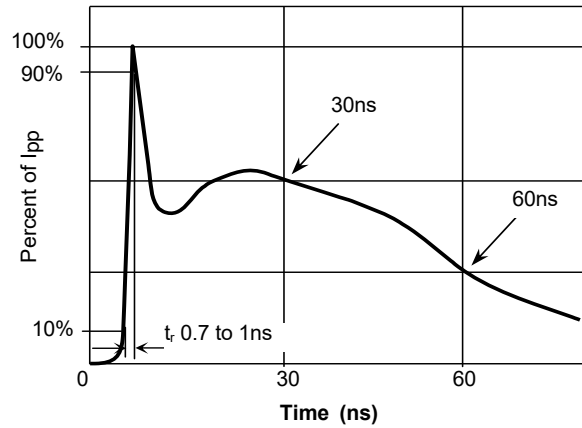
Fig.6 IEC61000-4-2 -8kV Contact Discharge
